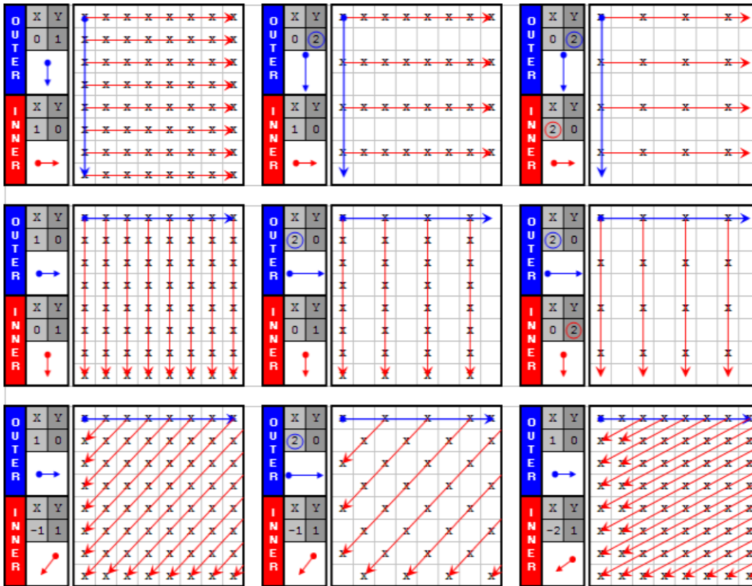
Figure: Local Loop Walking Patterns
