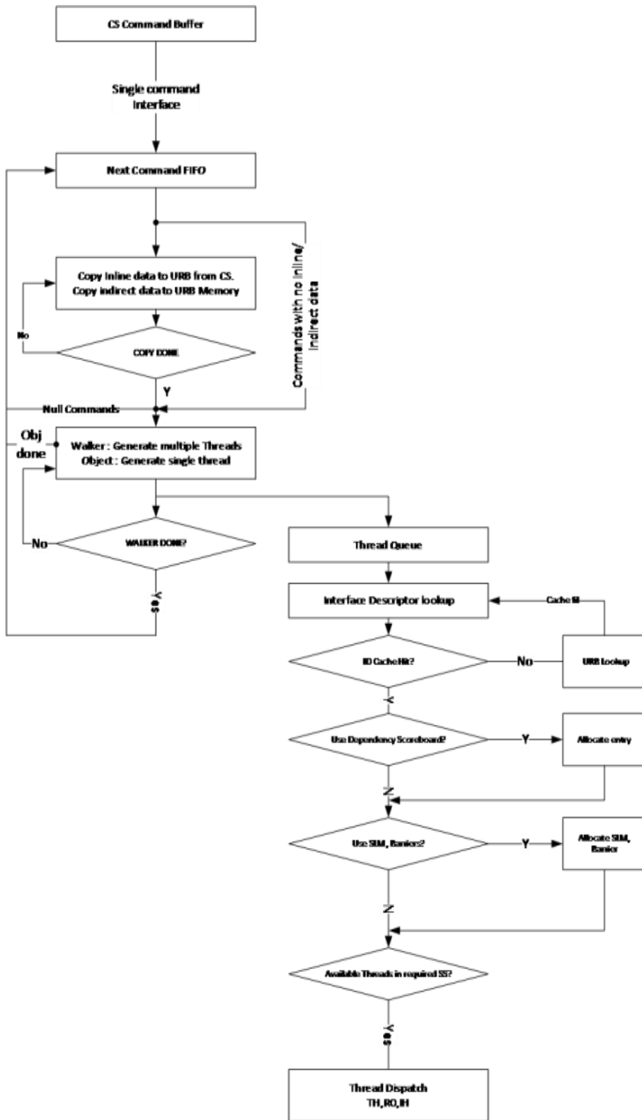
Figure: Thread Lifecycle Process
