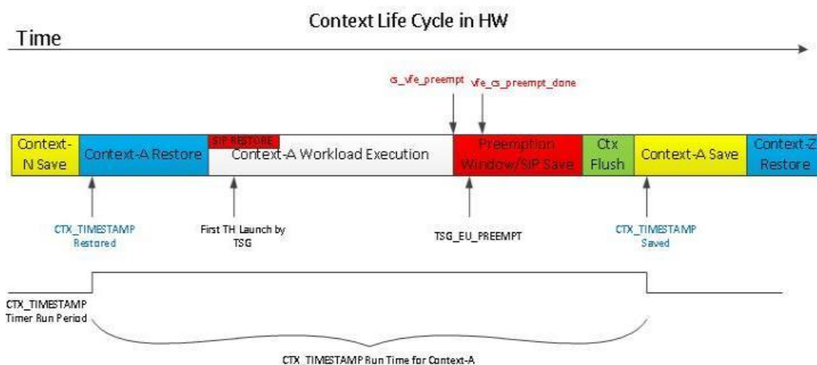
Fig: CS_CTX_TIMESTAMP functionality during context execution
