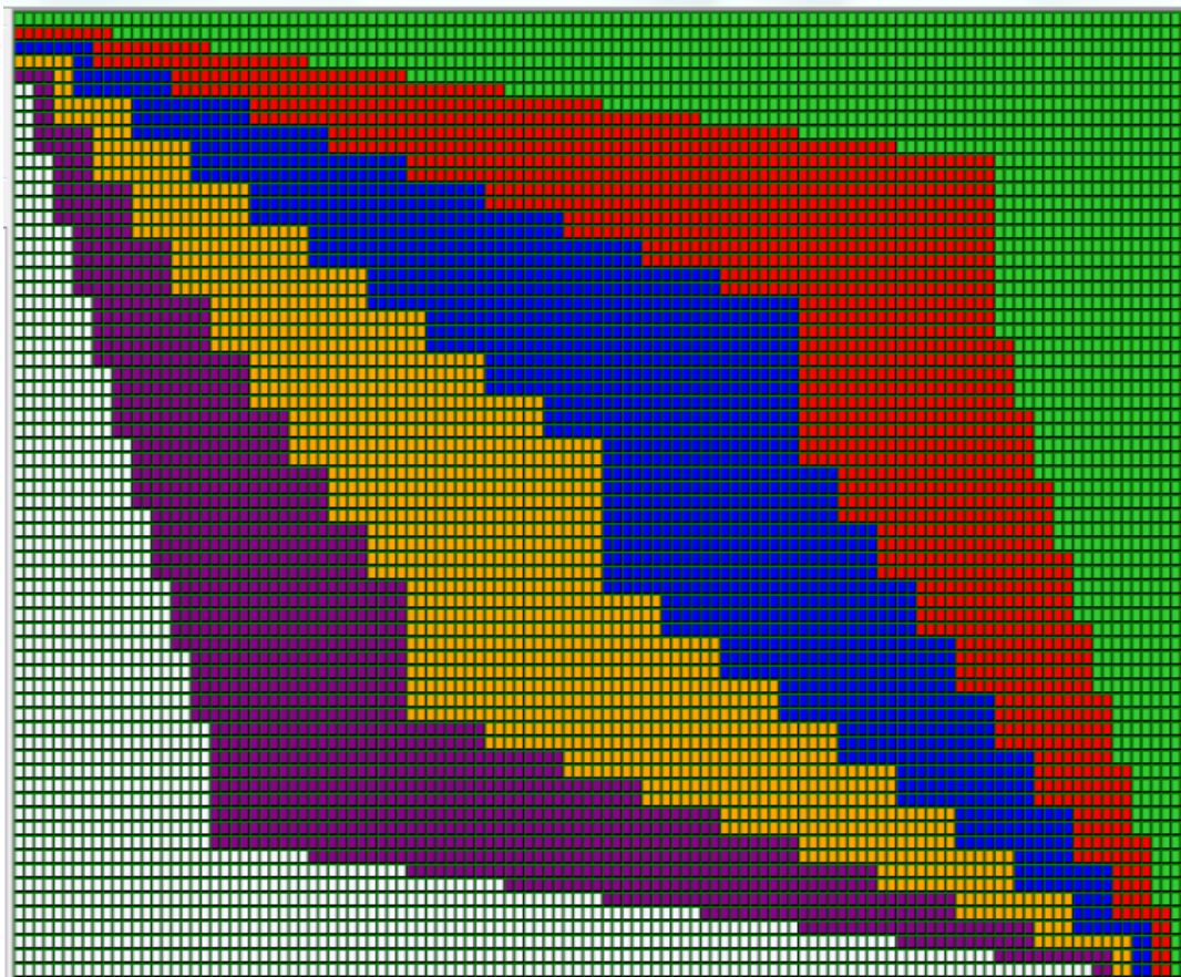
Figure: Splitting a Wavefront Between Six Segments
